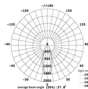
light distribution curve values
