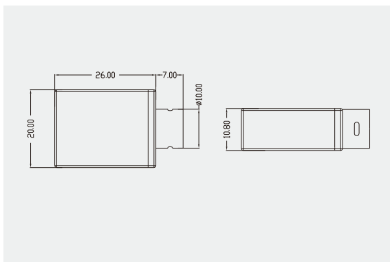
Screwless assembly end cap
