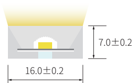
Unit: mm Cross section
