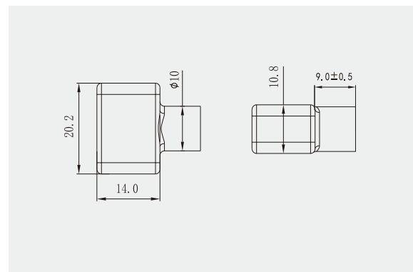
External hydraulic end cap
