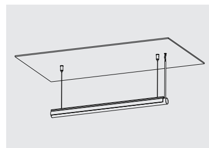
Drill 8–12mm holes on the mounting surface of the input end of the light body, pull out the wires and connect them with the input wires of the light bar.
