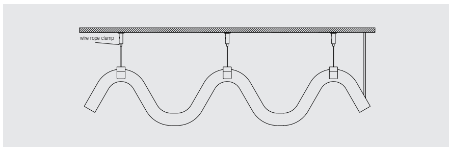
Adjust the length of the wire rope to a suitable length by means of the wire rope locking device on the wire rope to complete the installation.
