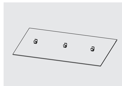
Finish fixing the other clips in turn. Note: Install at least 3pcs of clips per meter of light bar.
