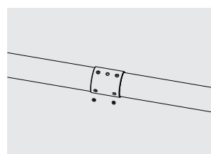
Fasten with self-tapping screws, 4 screws for each plug.
