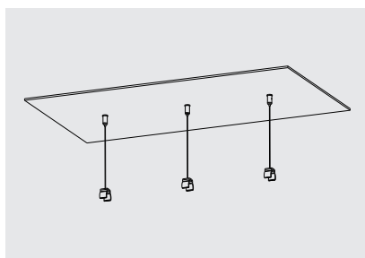
Install the rest of the lanyards and cable locks in turn.
