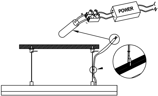
④ Connect the power supply and complete the installation.
